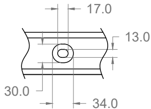
Hole Detail
