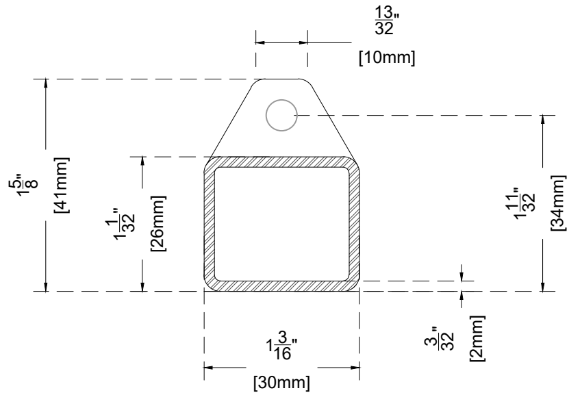
VUE DE FACE- front view
