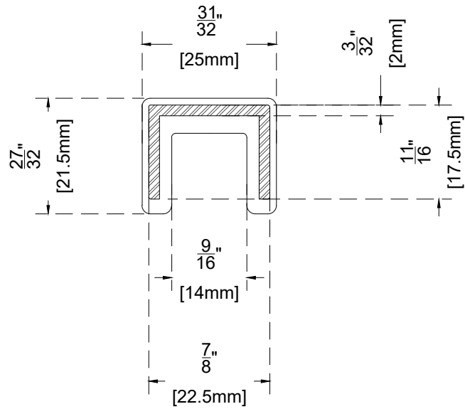
VUE DE FACE- front view
