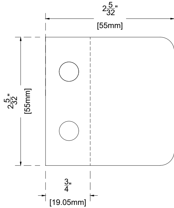
VUE DE FACE- SANS PLAQUE front view without bottom plate
